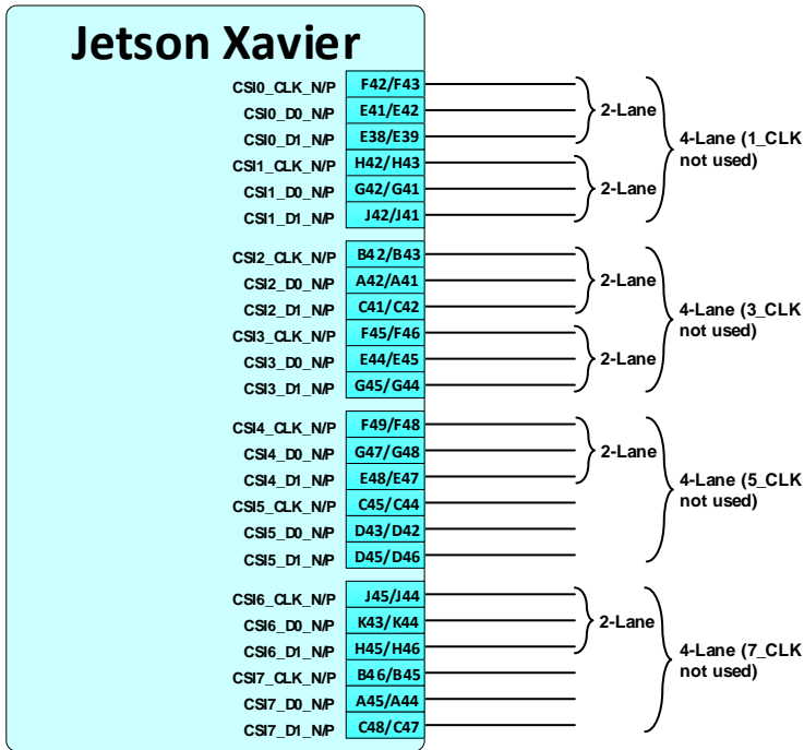
Figure 14: Camera CSI Connections (D-PHY)
