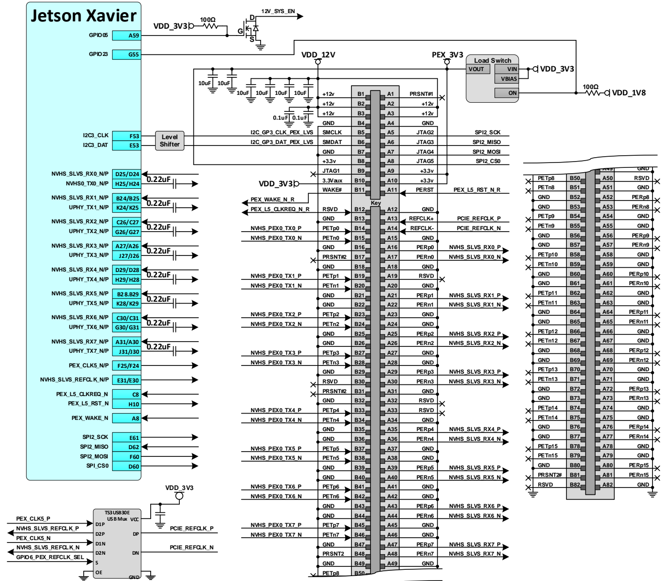
Figure 6. PCIe x16 Connector Connections
