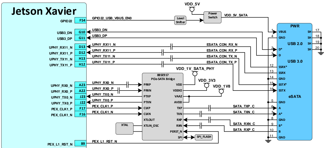
Figure 8. eSATA Connections
