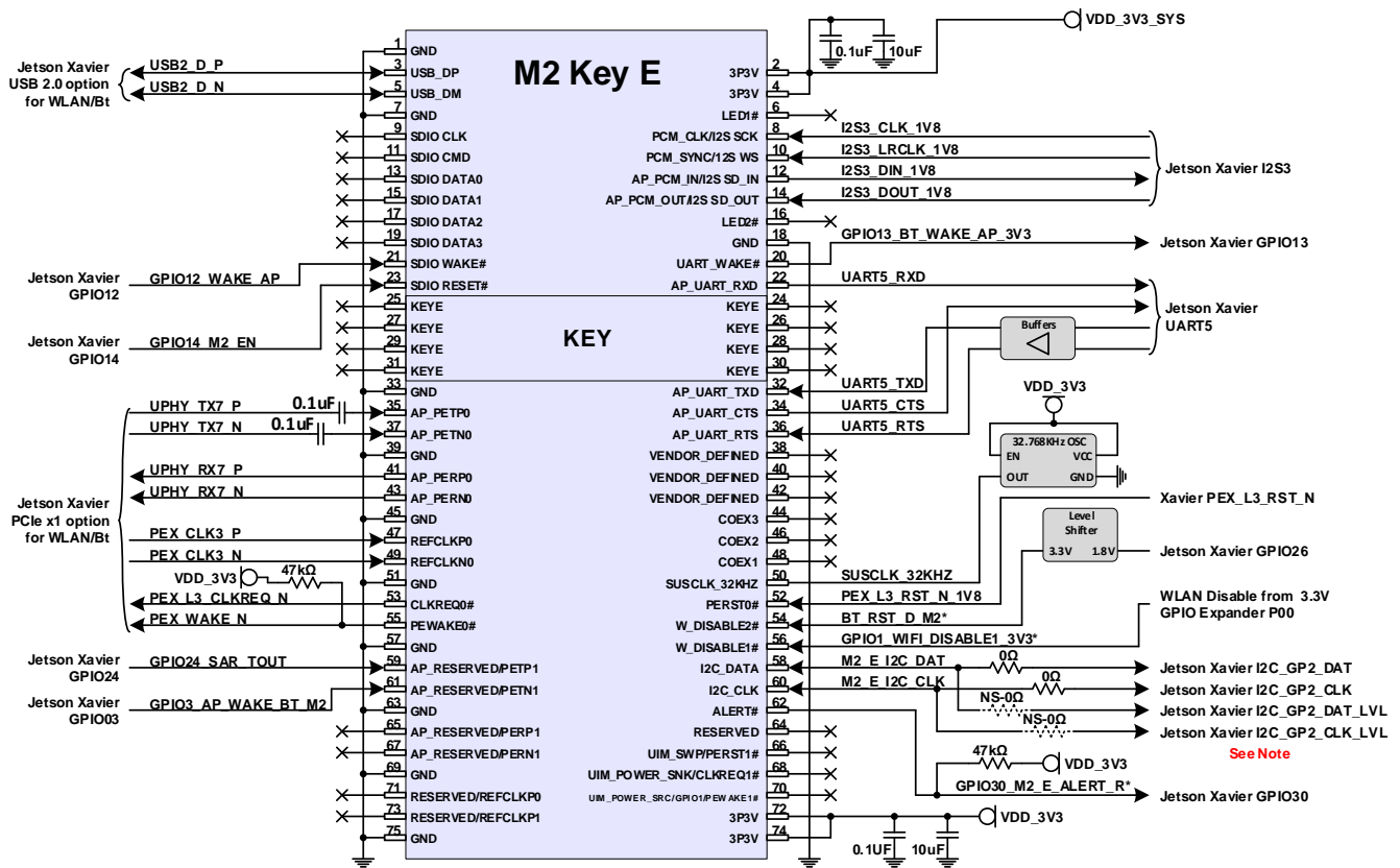
Figure 9. M.2 Key E Connections
