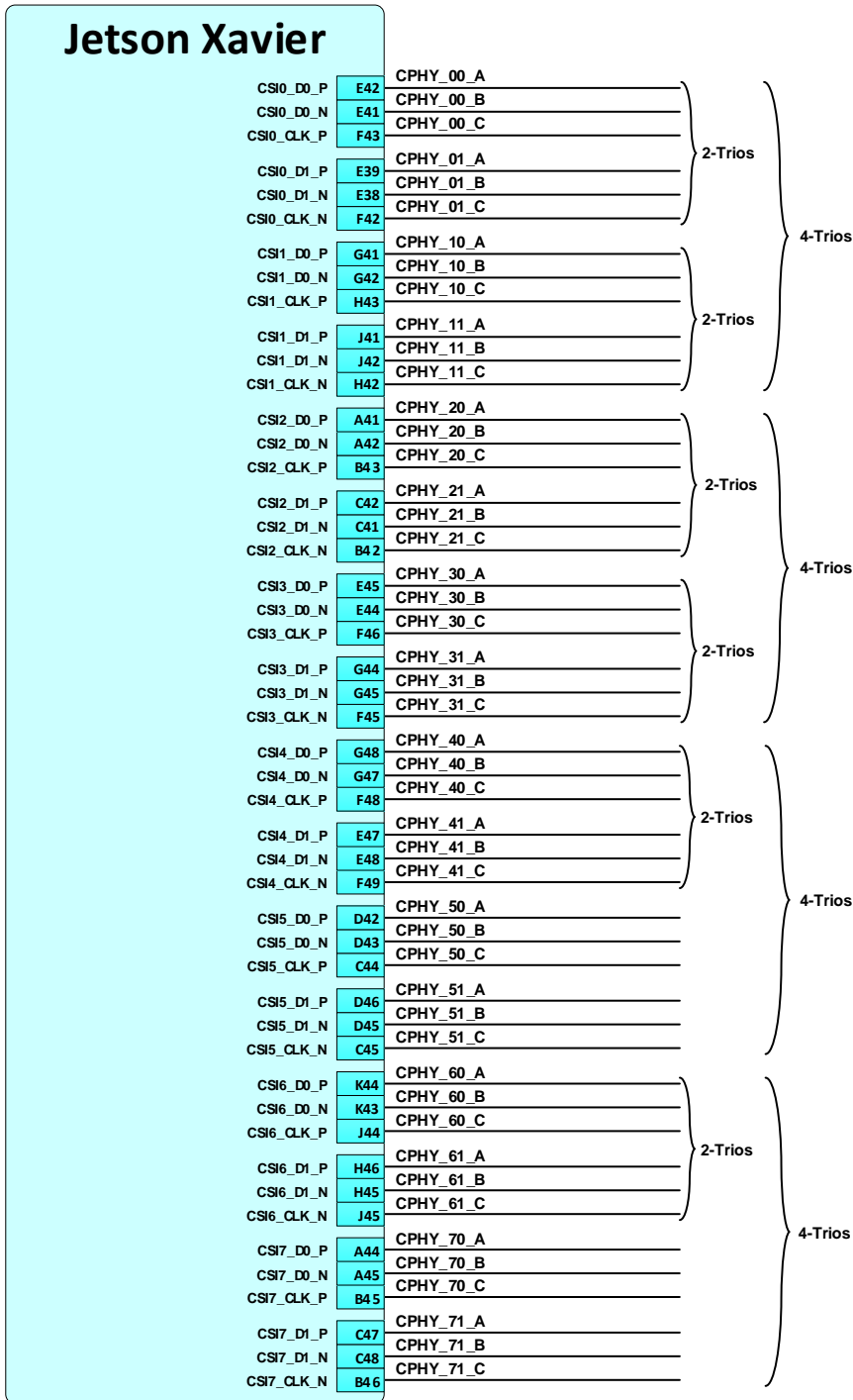
Figure 13: Camera CSI Connections (C-PHY)
