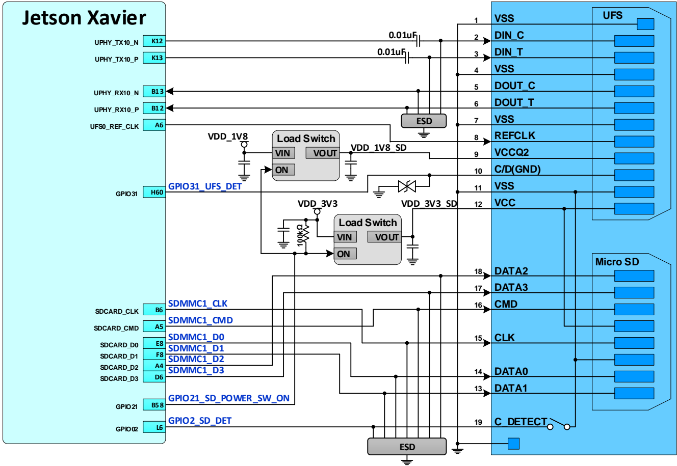
Figure 7. UFS / SD Card Connections
