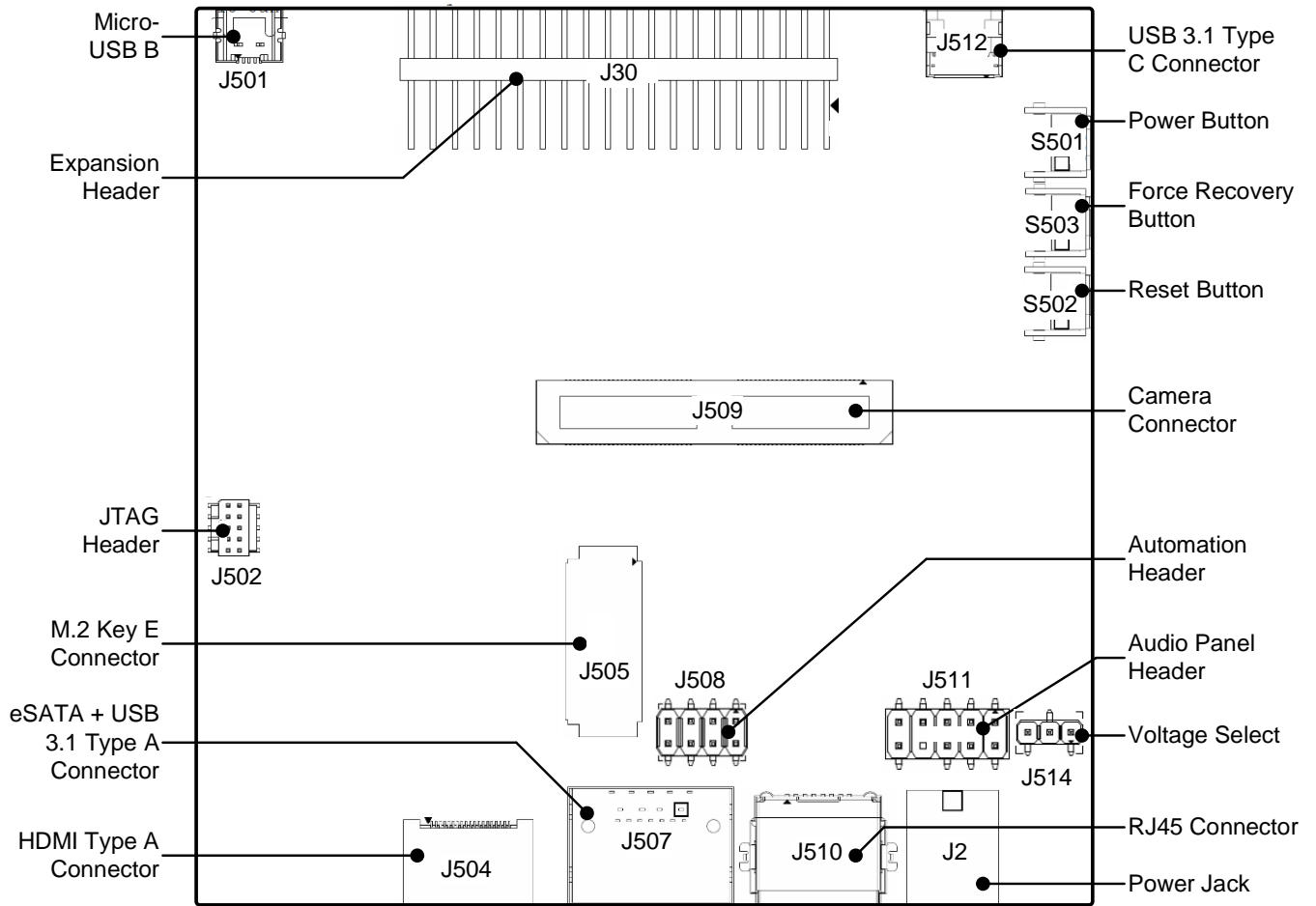
Figure 2. Jetson Xavier Carrier Board Placement (Bottom View)
