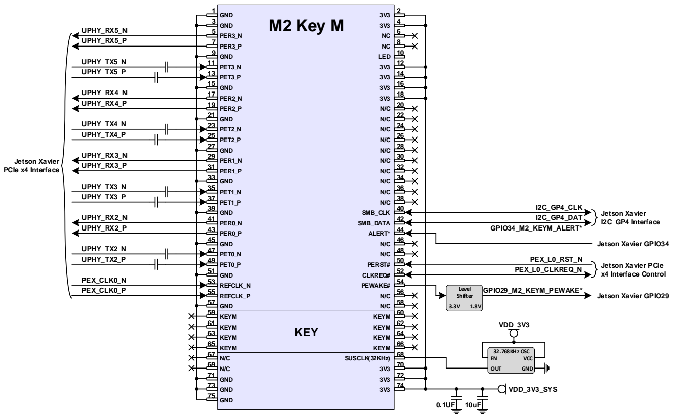
Figure 10. M.2 Key M Connections
