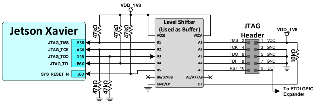
Figure 12. JTAG Header Connections
