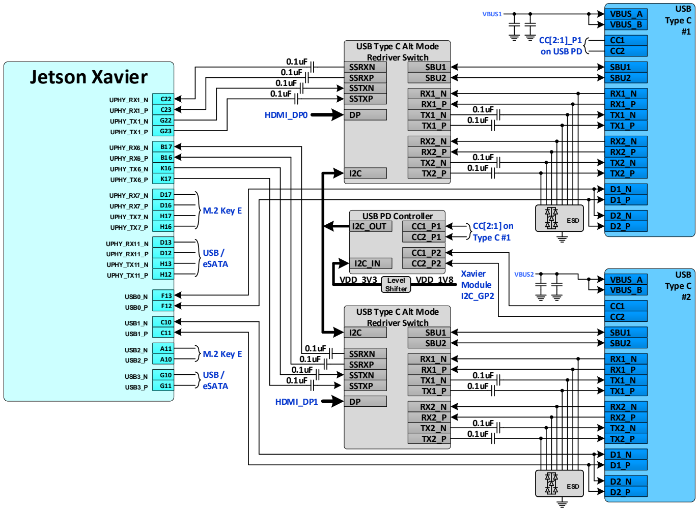
Figure 3. USB Type C Port Connections
