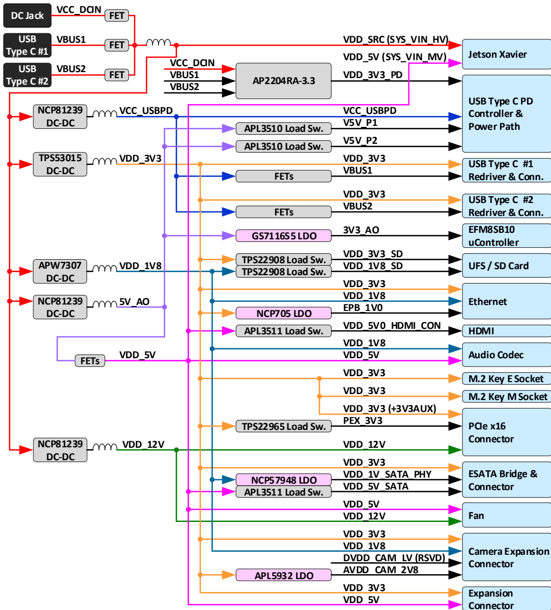
Figure 16. Interface Connector Power Diagram
