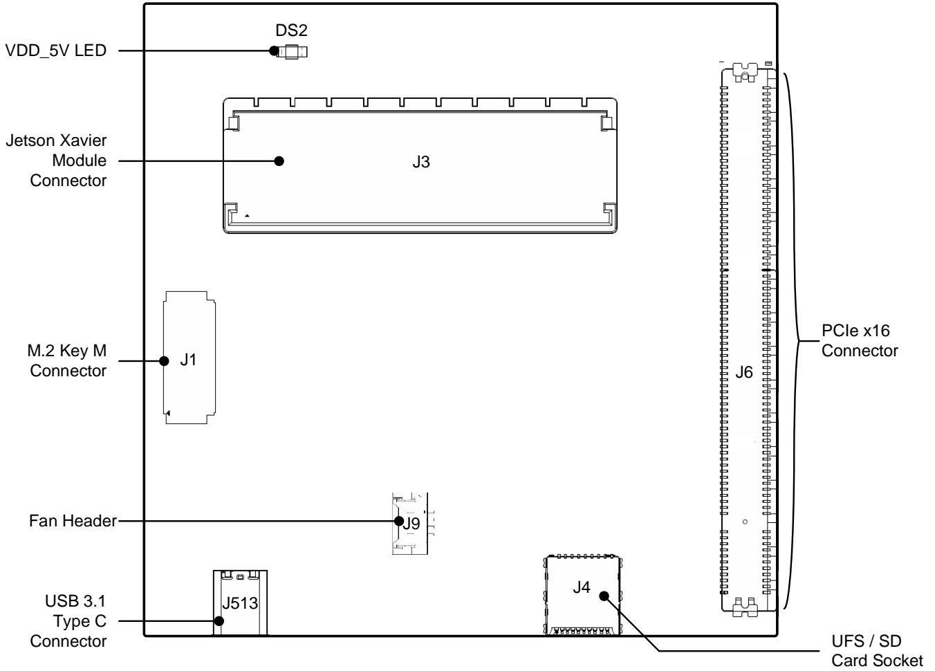
Figure 1. Jetson Xavier Carrier Board Placement (Top View)
