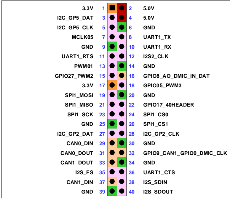
Figure 15. Expansion Header (Top View)
